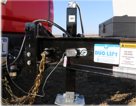
2-5/6" ADJUSTABLE BALL COUPLER, SAFETY CHAINS AND 7-WAY RV CONNECTOR
